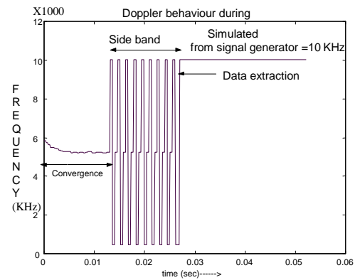
Fig.5 Performance of Sideband detection and Data Extraction algorithms
