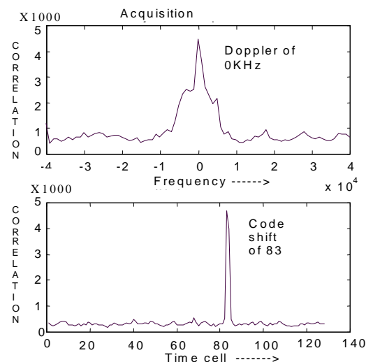
Fig.3 Acquisition algorithm performance in both Frequency and Time domain
