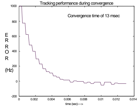
Fig.4 Carrier Lock Loop filter performance during Convergence
