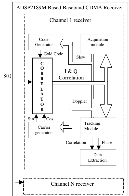
Fig. 2 Functional diagram of ADSP2189M based Multi channel CDMA Baseband receiver
