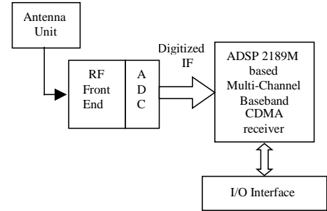
Fig. 1 Interfacing diagram for Multi- Channel Baseband CDMA receiver
